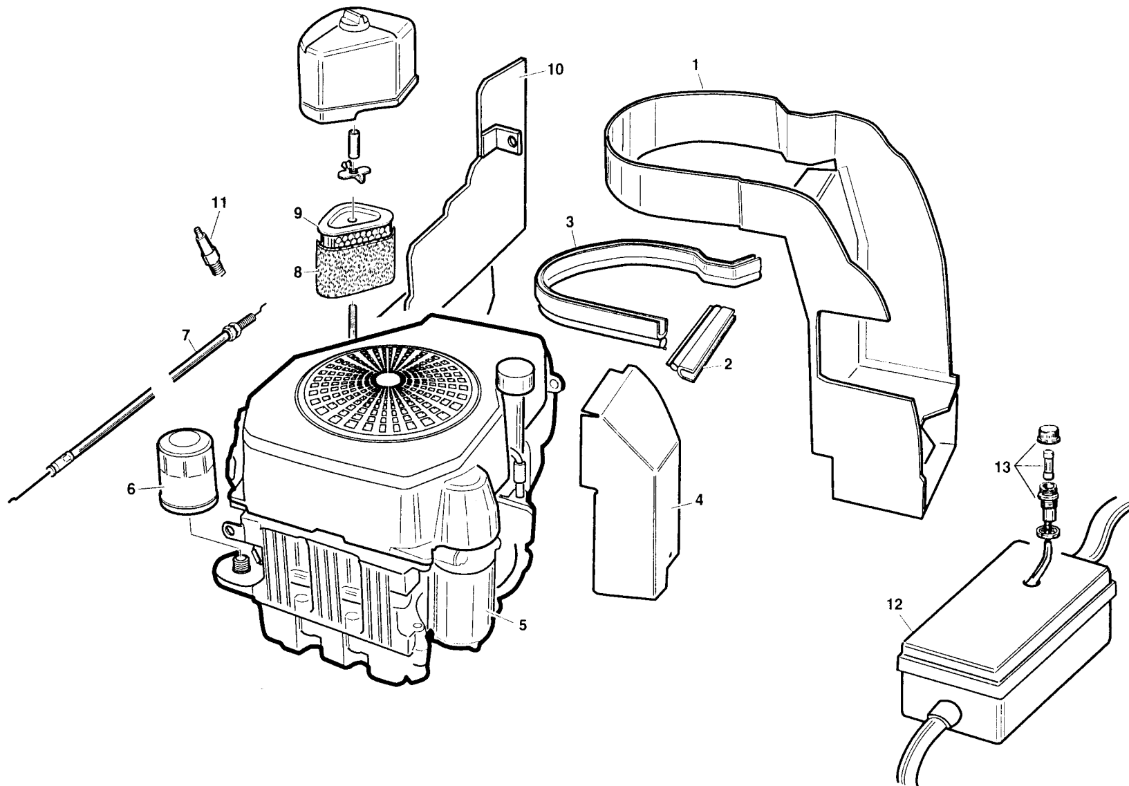
Tav. 07/4 - 15,5HP KOHLER NEW - B 21/2/99
